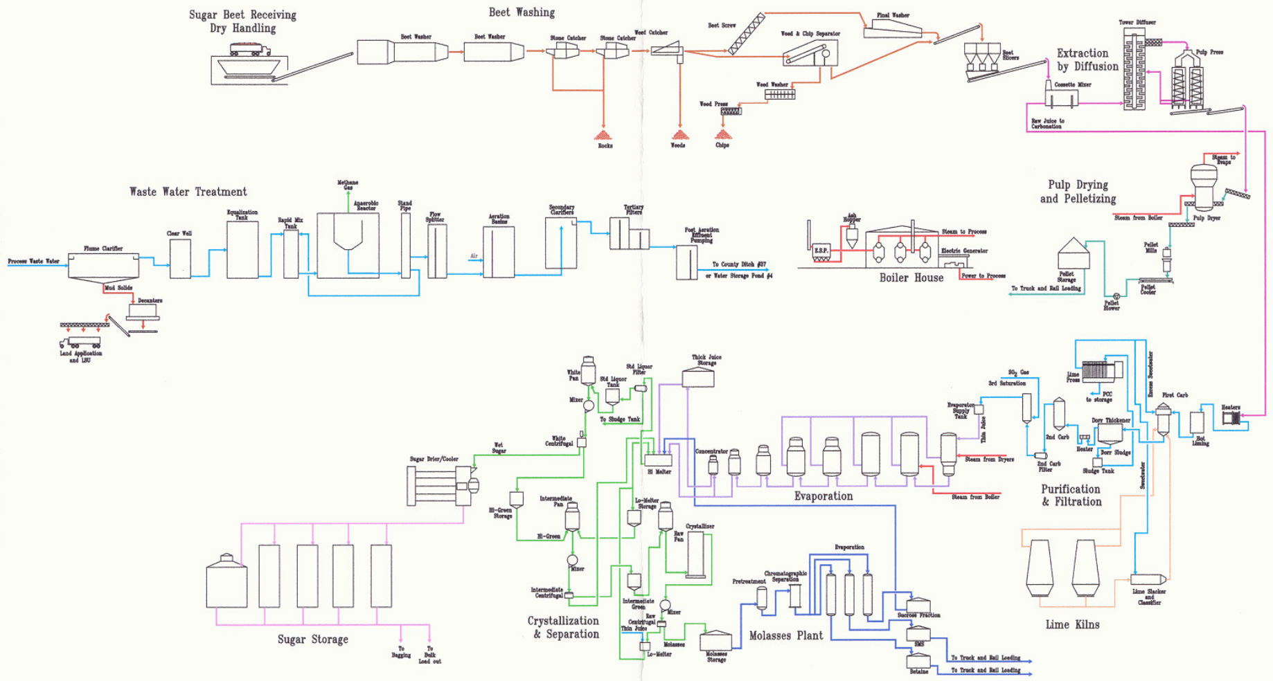
PROCESS FOR BEET SUGAR BASIC FLOW DIAGRAM
